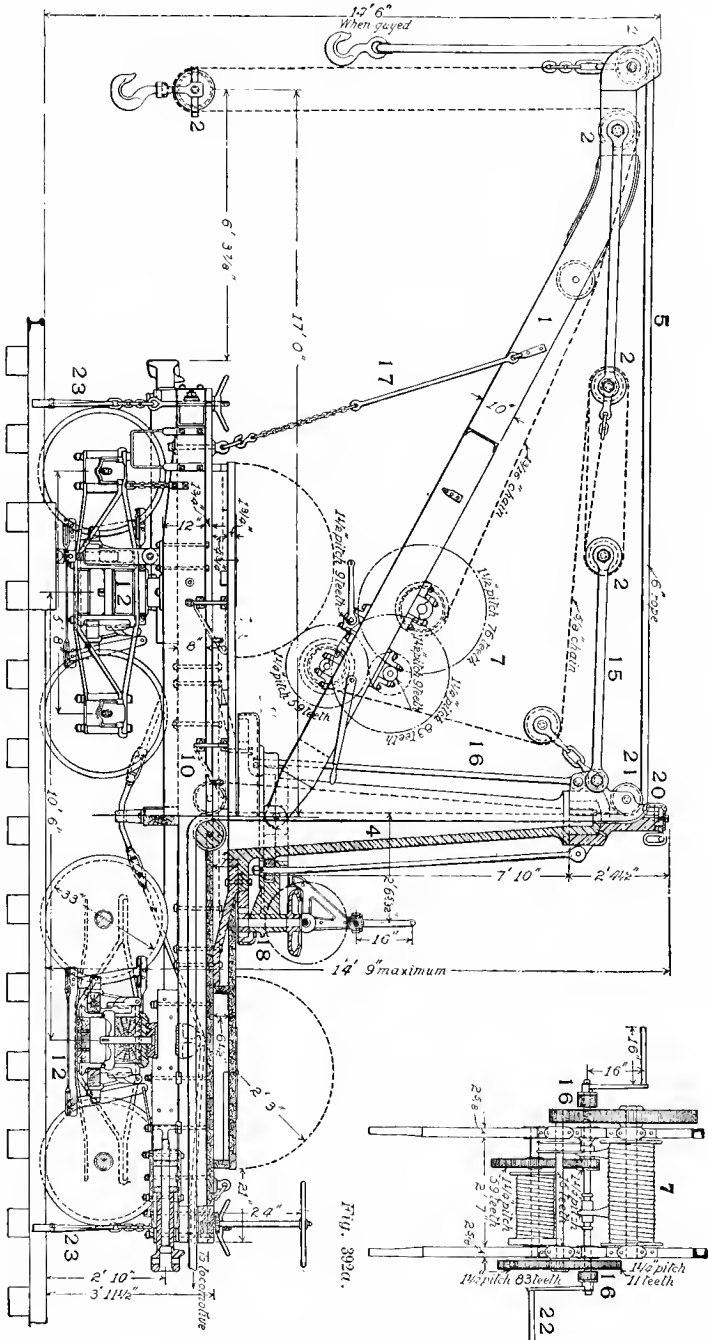
Fig. 392. Side Elevation. HAND DERRICK CAR. BALTIMORE & OHIO RAILROAD. Capacity, 20,000 lbs. Sweep, 31 ft.
